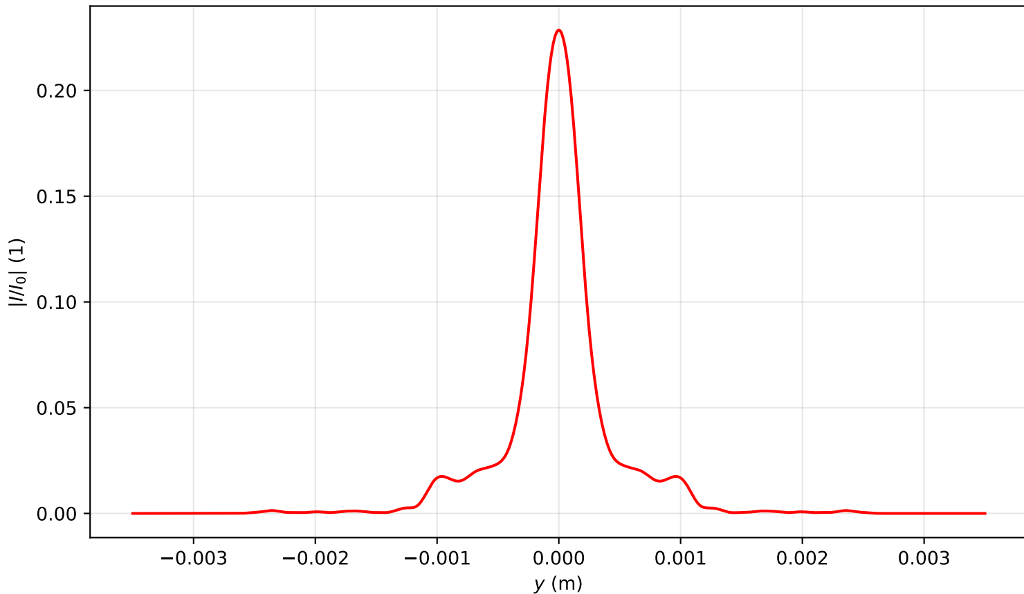
Intensity profile I(x=0, y, z=2.866)/I_0 , P_{in}=16.0\text{Pcr} , artificial time
