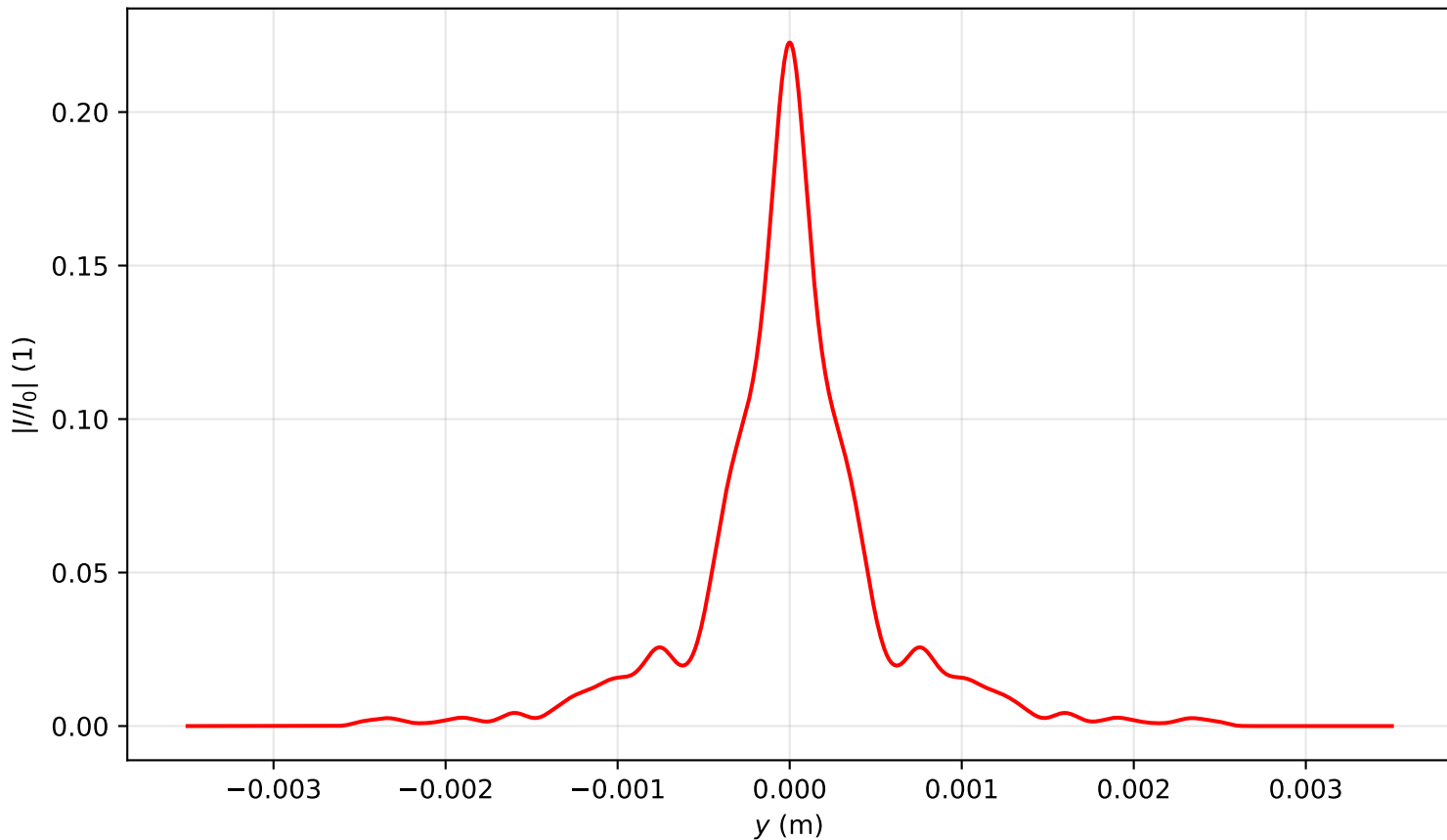
Intensity profile I(x = 0, y, z = 3.105)/I_0 , P_{in}=16.0P_{cr} , artificial time
