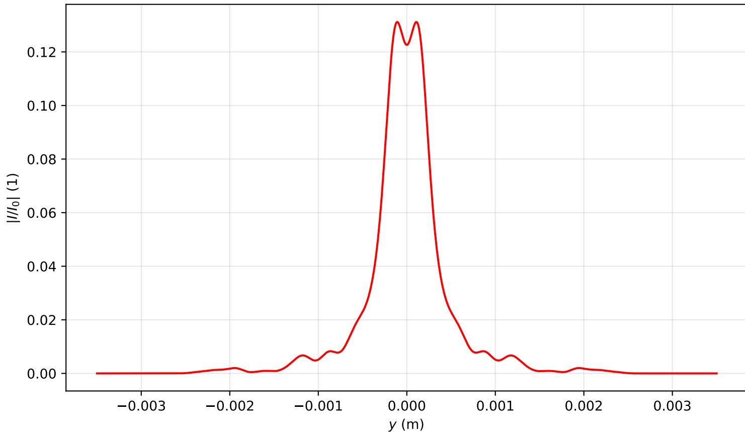
Intensity profile I(x=0, y, z=3.344)/I_0 , P_{in}=16.0P_{cr} , artificial time
