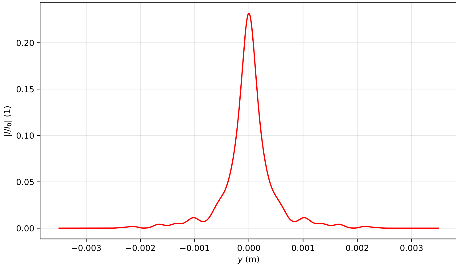
Intensity profile I(x=0, y, z=3.821)/I_0 , P_{in}=16.0P_{cr} , artificial time
