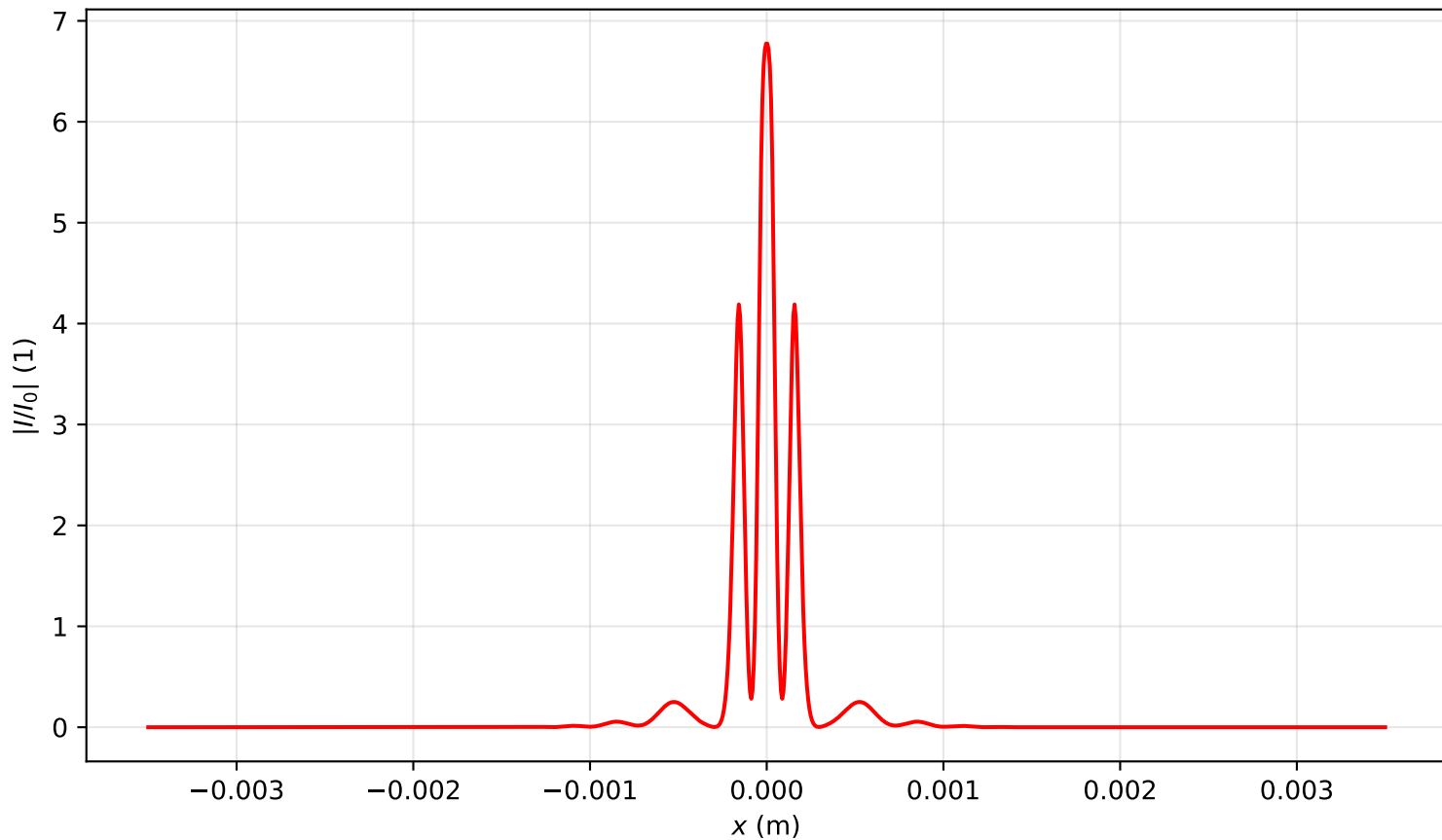
Intensity profile I(x, y = 0, z = 0.478)/I_0 , P_{in}=16.5P_{cr} , artificial time
