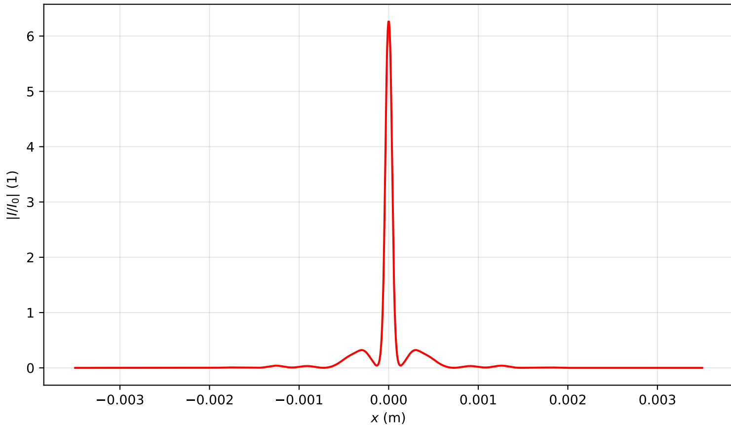
Intensity profile I(x, y = 0, z = 0.955)/I_0 , P_{in}=16.5P_{cr} , artificial time
