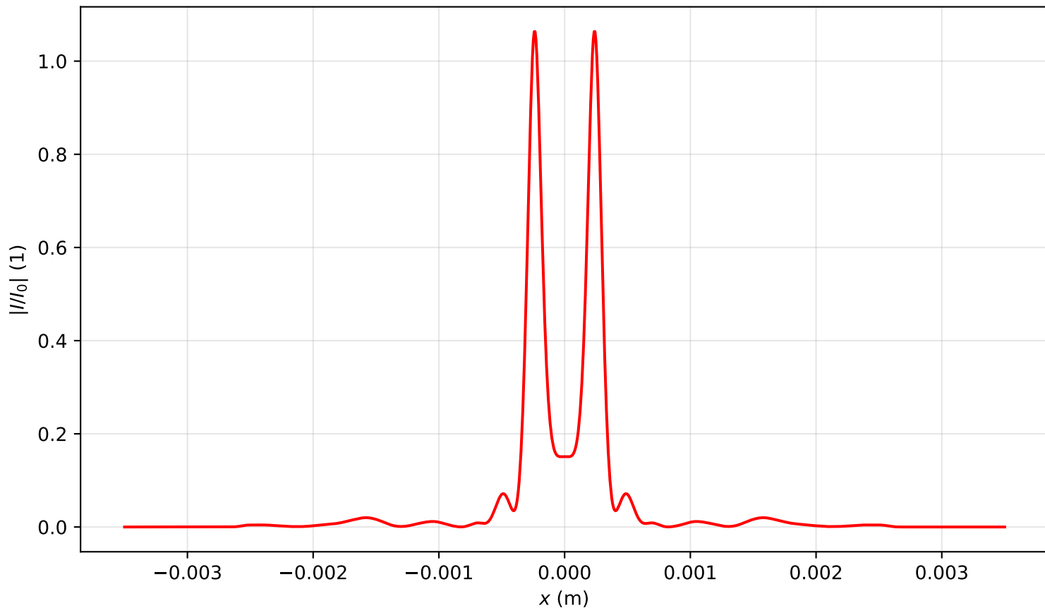
Intensity profile I(x, y = 0, z = 1.194)/I_0 , P_{in}=16.5P_{cr} , artificial time
