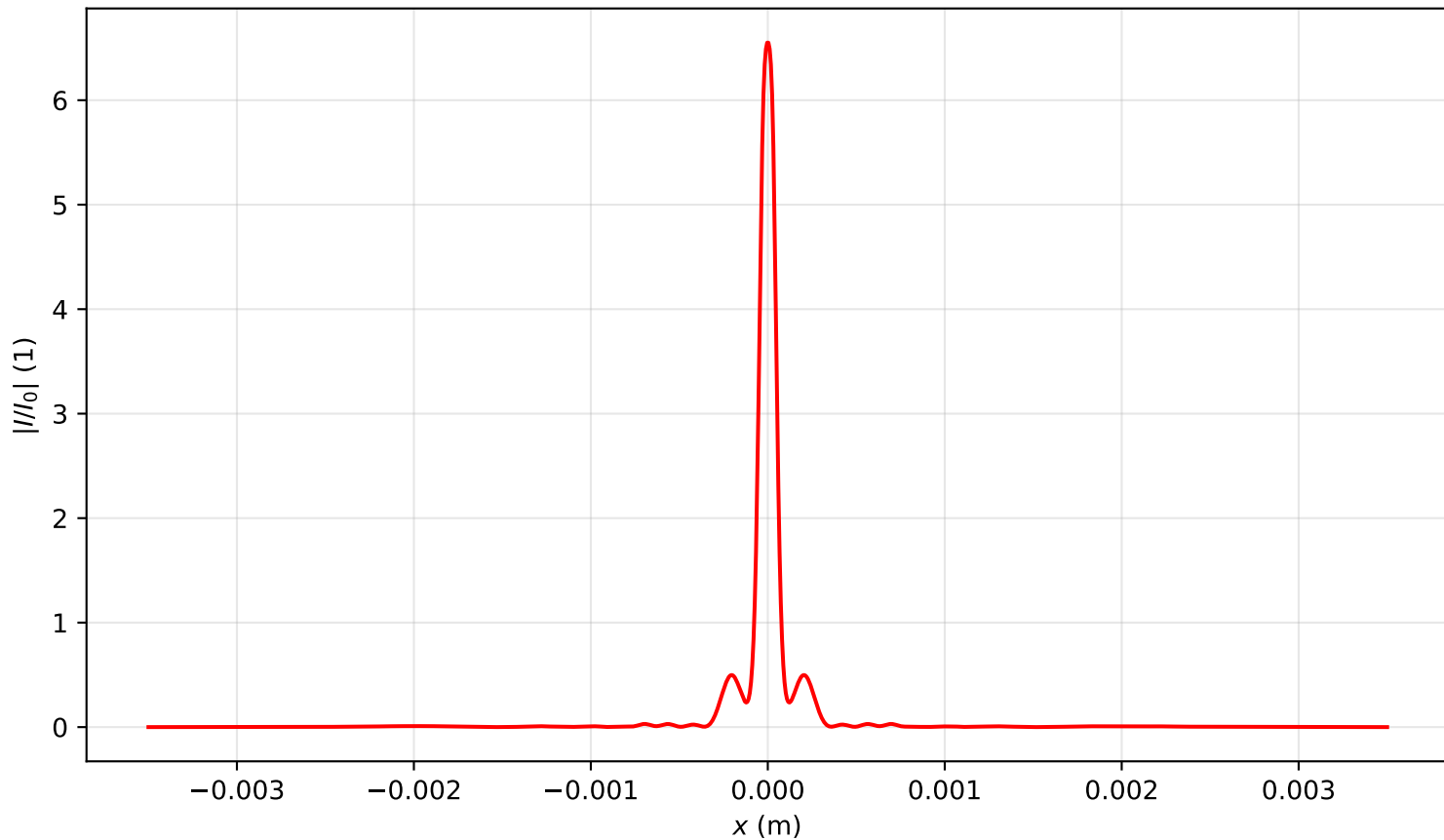
Intensity profile I(x, y = 0, z = 1.433)/I_0 , P_{in}=16.5P_{cr} , artificial time
