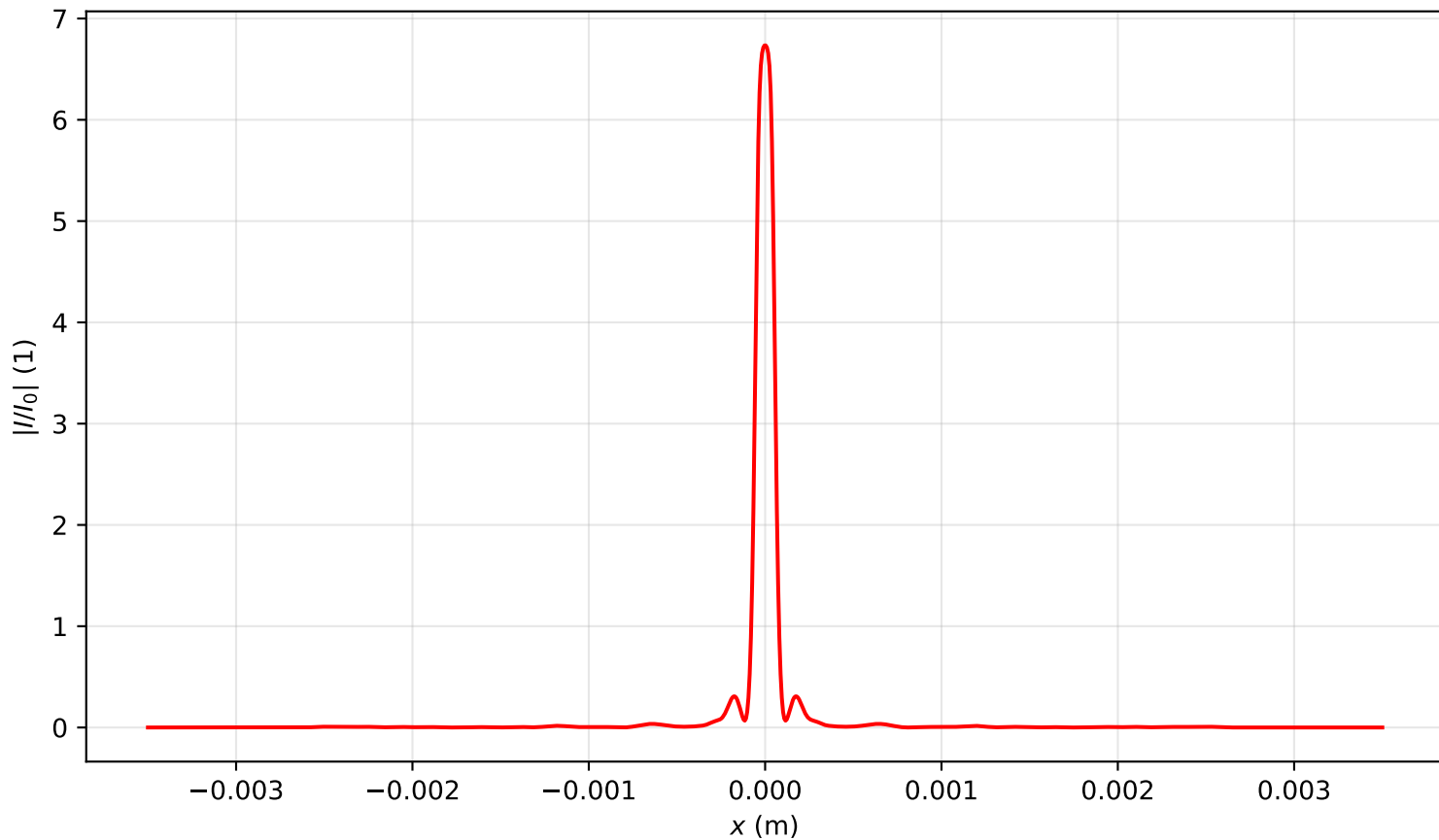
Intensity profile I(x, y = 0, z = 1.672)/I_0 , P_{in}=16.5P_{cr} , artificial time
