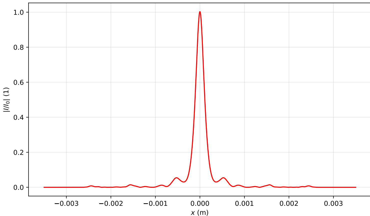
Intensity profile I(x, y = 0, z = 1.911)/I_0 , P_{in}=16.5P_{cr} , artificial time
