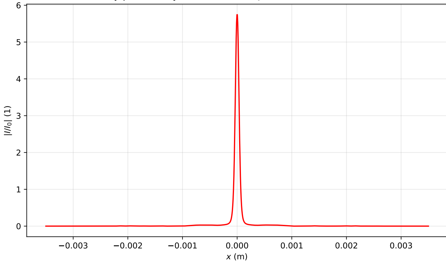
Intensity profile I(x, y = 0, z = 2.149)/I_0 , P_{in}=16.5P_{cr} , artificial time
