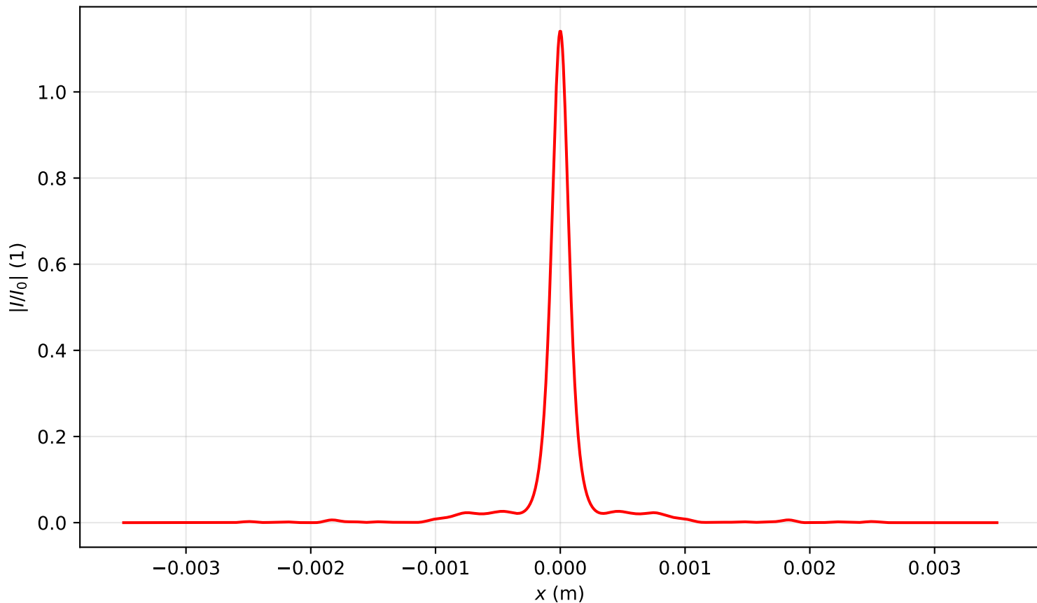
Intensity profile I(x, y = 0, z = 2.388)/I_0 , P_{in}=16.5P_{cr} , artificial time
