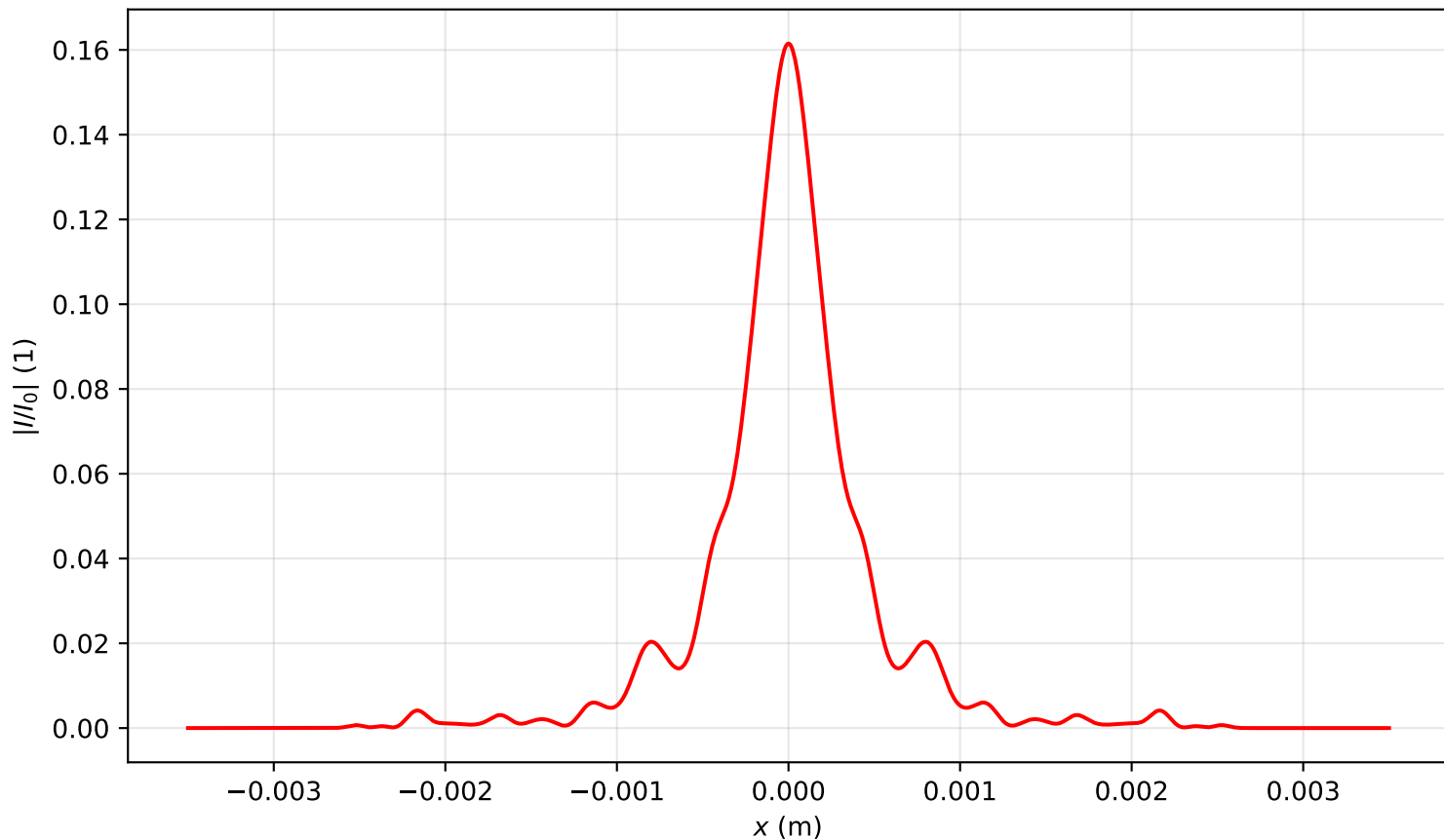
Intensity profile I(x, y = 0, z = 2.627)/I_0 , P_{in}=16.5P_{cr} , artificial time
