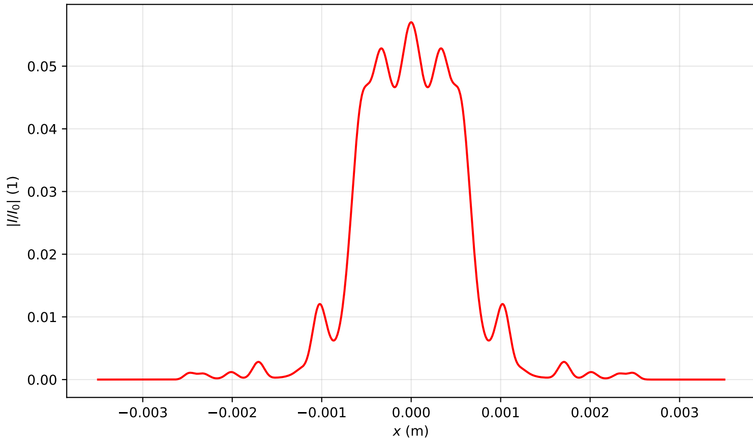
Intensity profile I(x, y = 0, z = 2.866)/I_0 , P_{in}=16.5P_{cr} , artificial time
