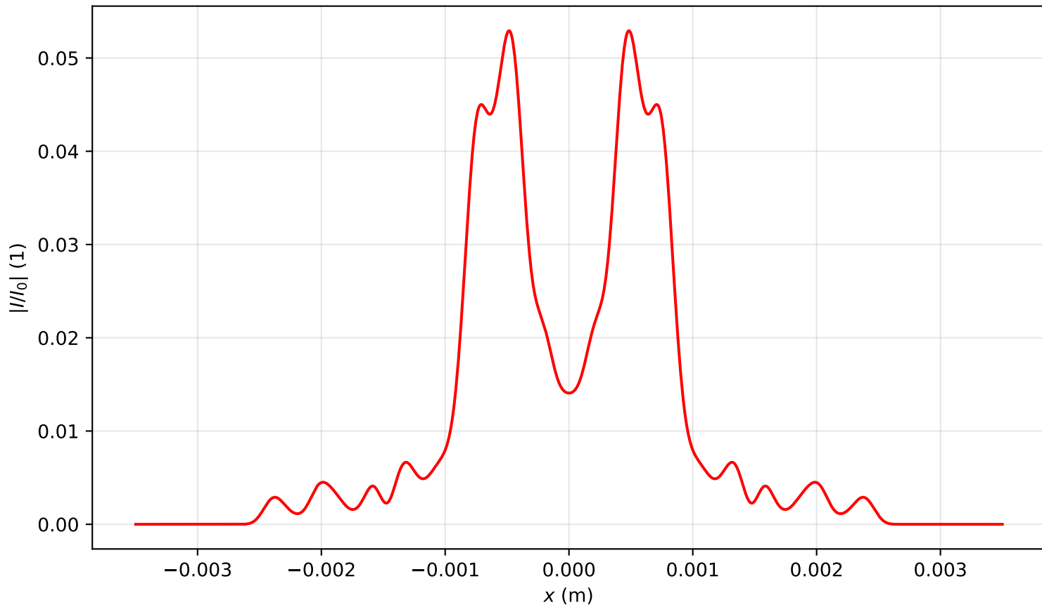
Intensity profile I(x, y = 0, z = 3.105)/I_0 , P_{in}=16.5P_{cr} , artificial time
