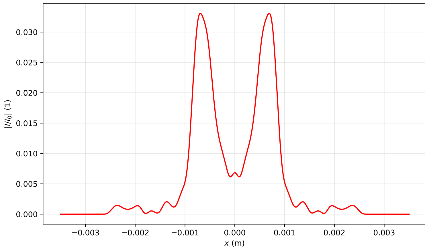
Intensity profile I(x, y = 0, z = 3.344)/I_0 , P_{in}=16.5P_{cr} , artificial time
