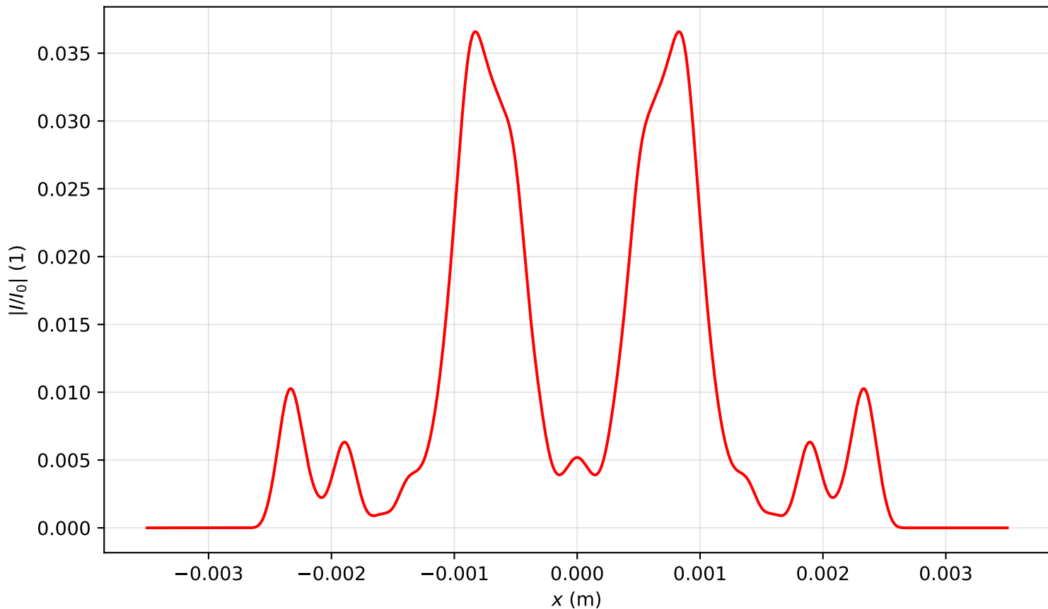
Intensity profile I(x, y = 0, z = 3.582)/I_0 , P_{in}=16.5P_{cr} , artificial time
