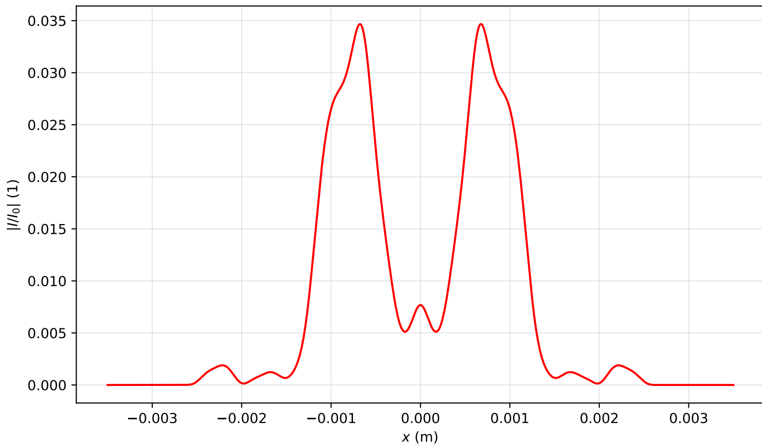
Intensity profile I(x, y = 0, z = 3.821)/I_0 , P_{in}=16.5P_{cr} , artificial time
