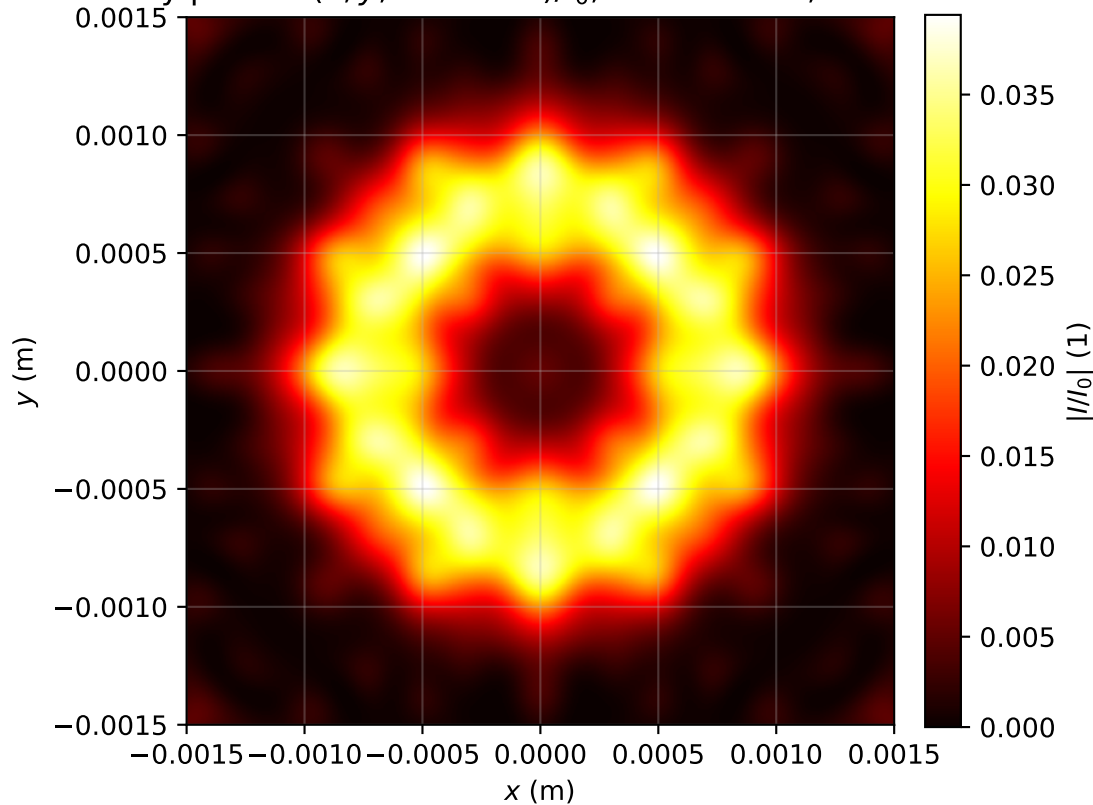
Intensity profile I(x, y, z = 3.582)/I_0 , P_{in}=16.5P_{cr} , artificial time
