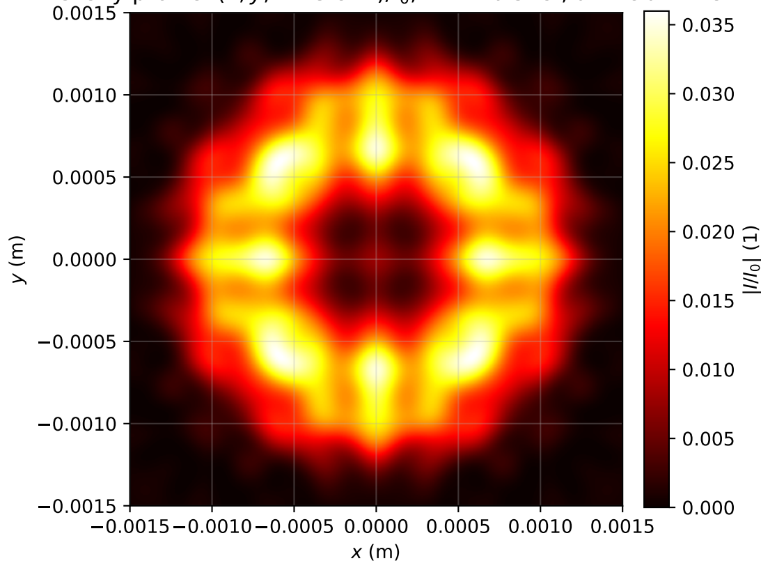
Intensity profile I(x, y, z = 3.821)/I_0 , P_{in}=16.5P_{cr} , artificial time
