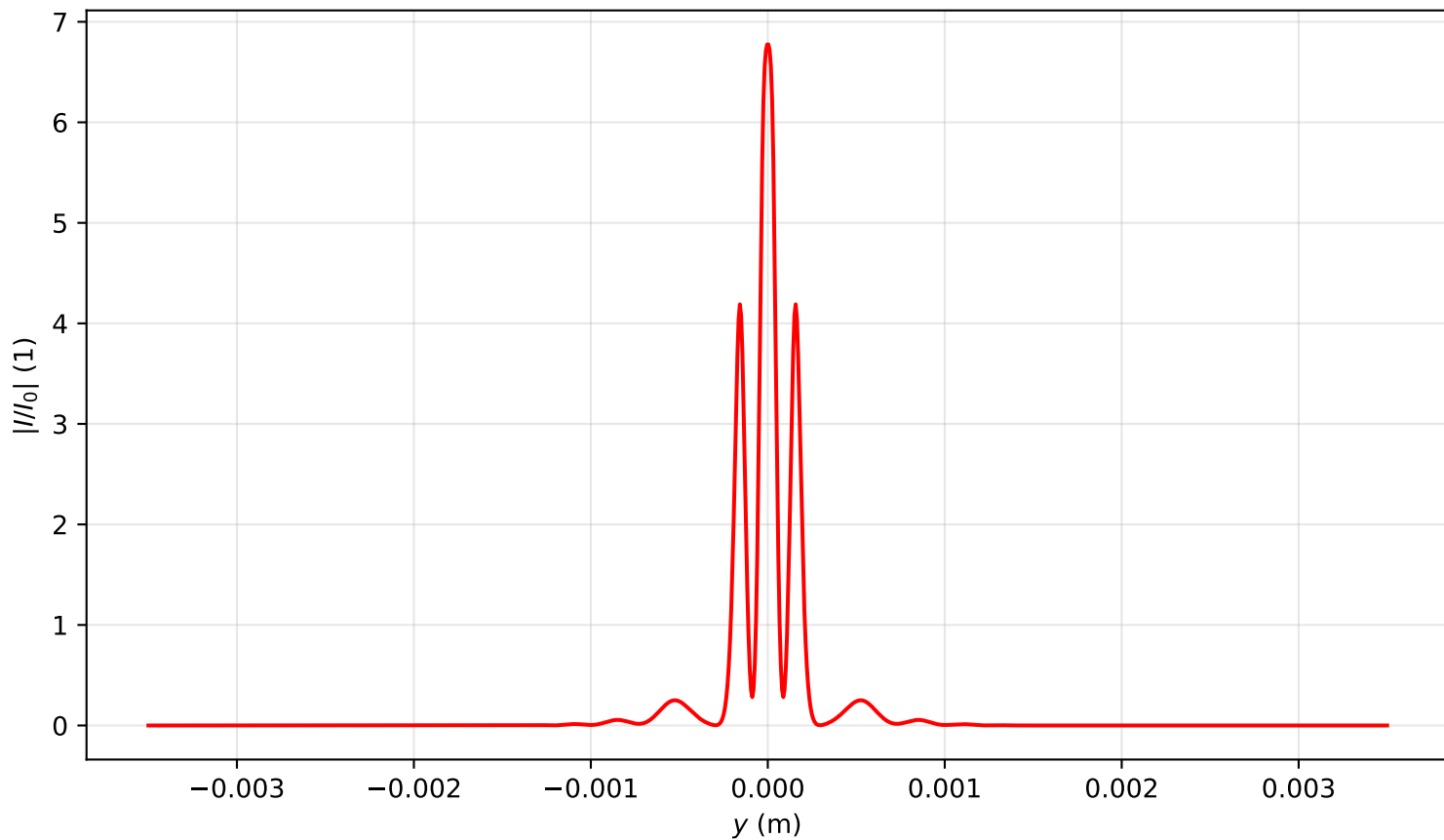
Intensity profile I(x=0, y, z=0.478)/I_0 , P_{in}=16.5P_{cr} , artificial time
