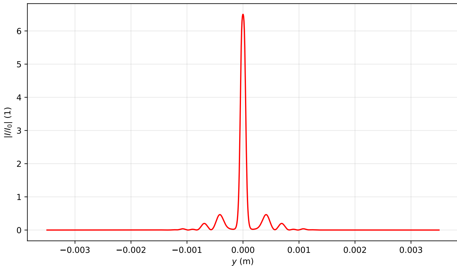
Intensity profile I(x=0, y, z=0.716)/I_0 , P_{in}=16.5P_{cr} , artificial time
