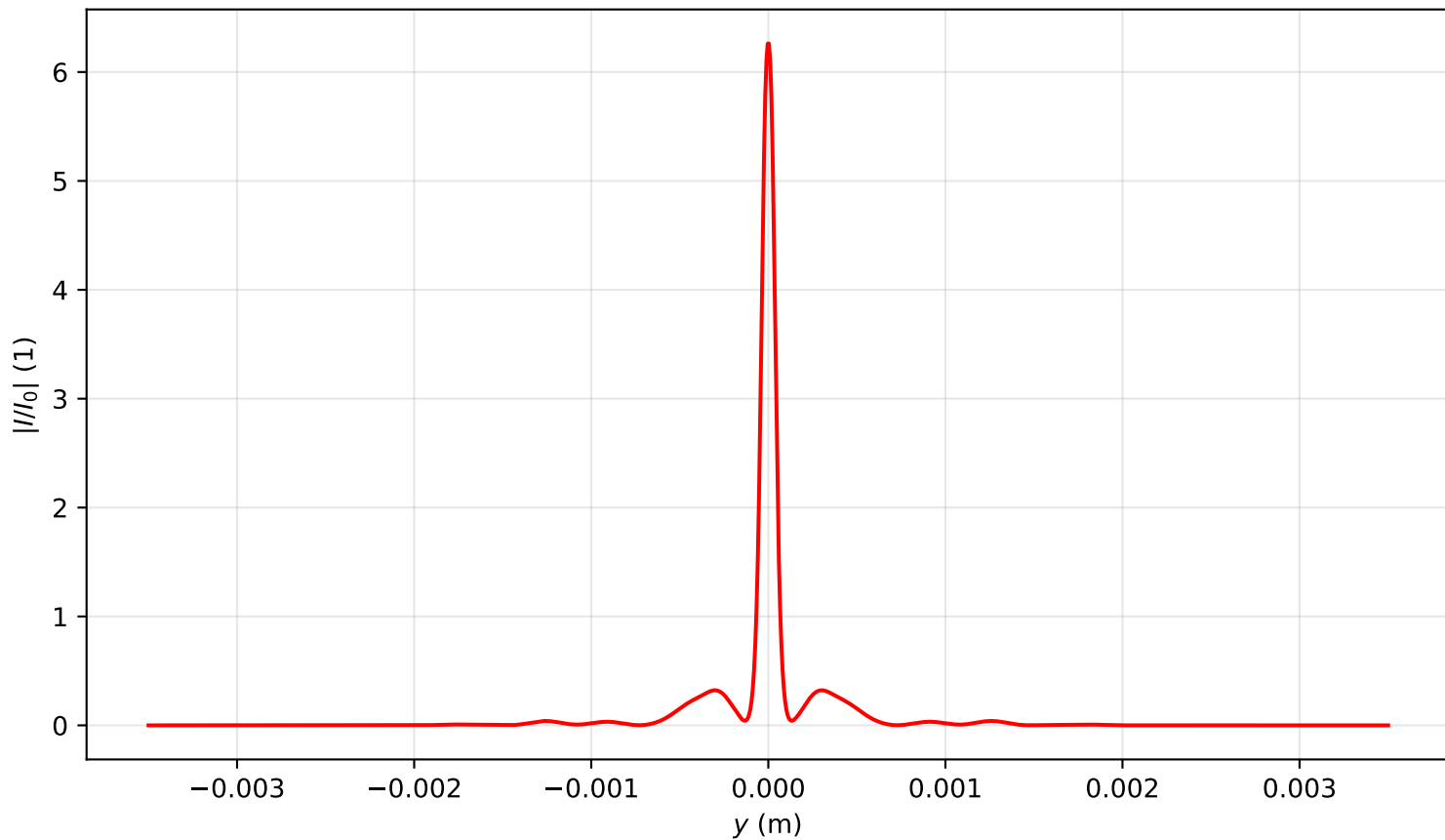
Intensity profile I(x=0, y, z=0.955)/I_0 , P_{in}=16.5P_{cr} , artificial time
