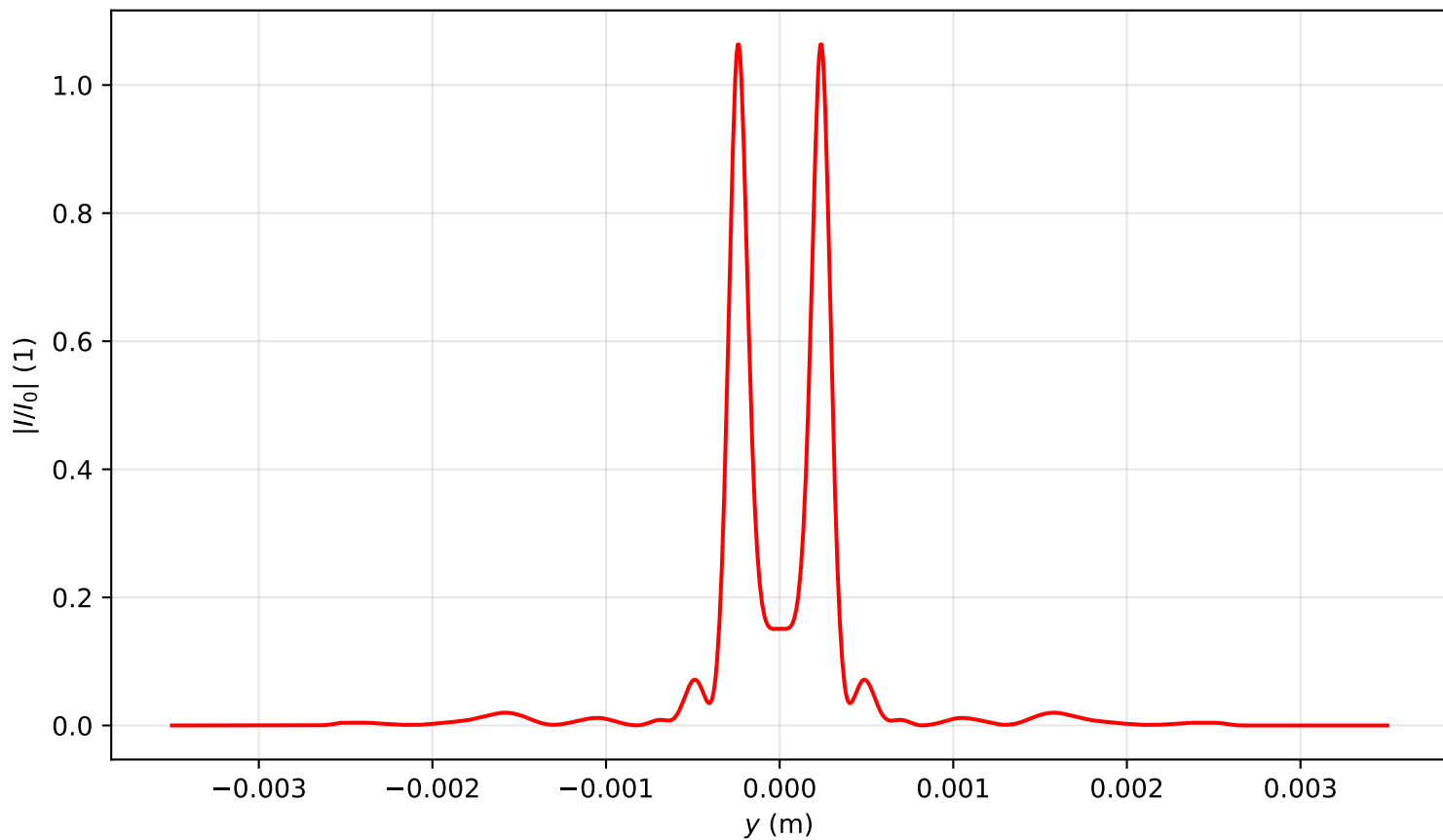
Intensity profile I(x=0, y, z=1.194)/I_0 , P_{in}=16.5P_{cr} , artificial time
