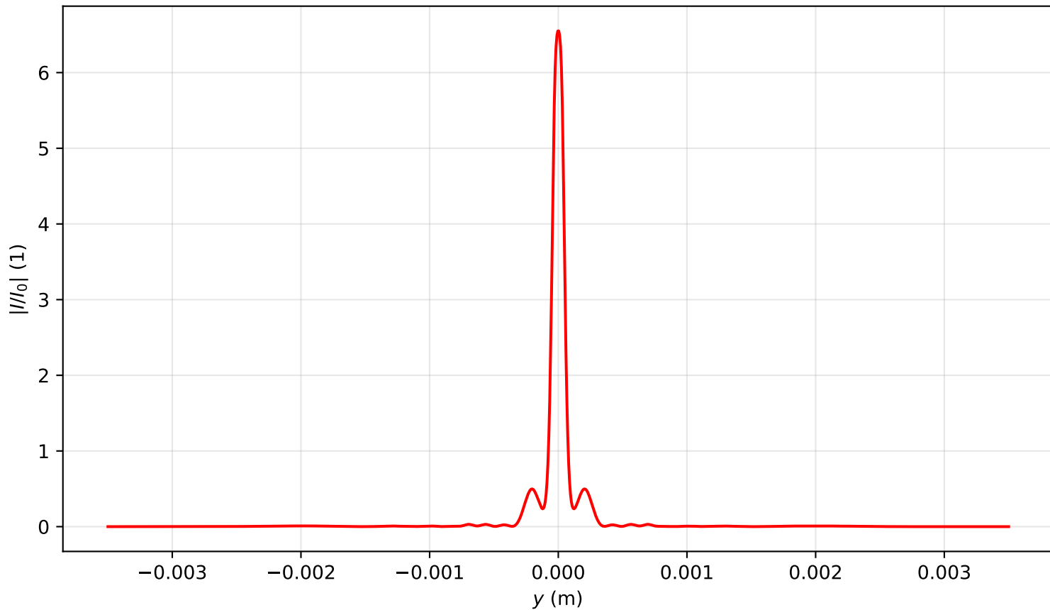
Intensity profile I(x=0, y, z=1.433)/I_0 , P_{in}=16.5P_{cr} , artificial time
