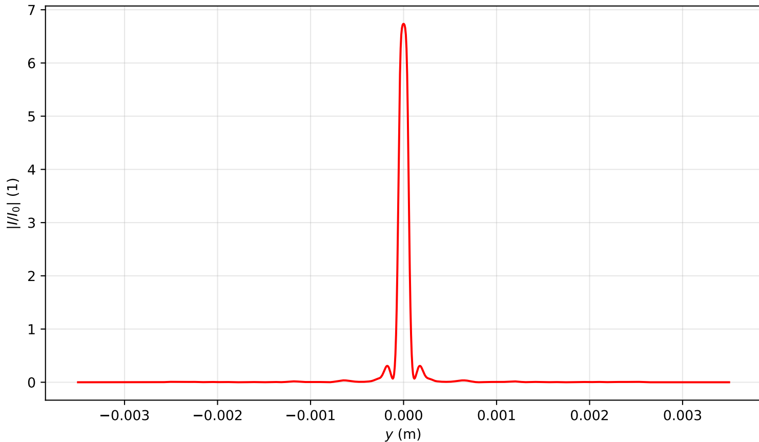
Intensity profile I(x=0, y, z=1.672)/I_0 , P_{in}=16.5P_{cr} , artificial time
