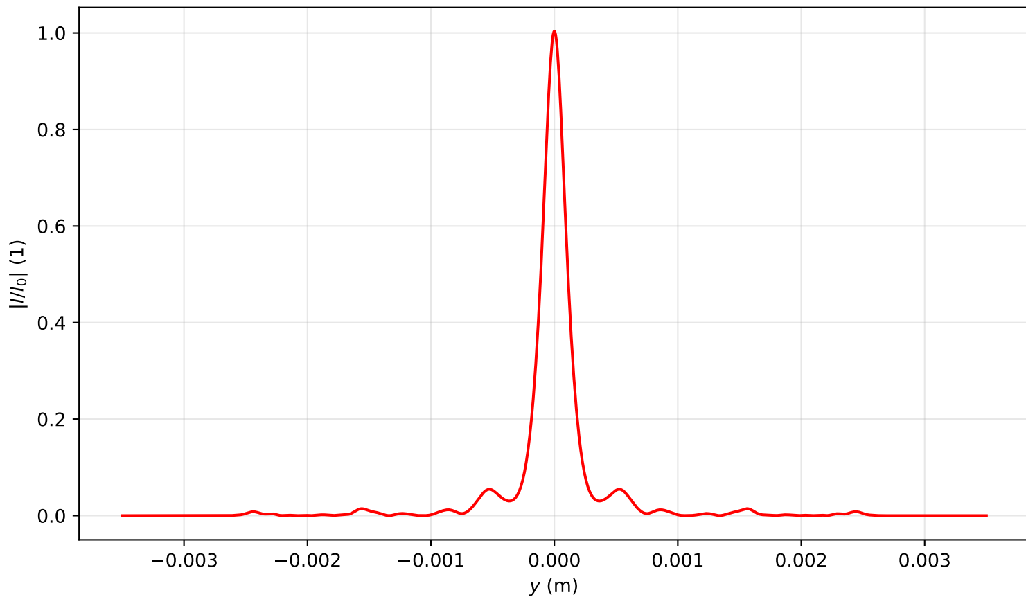
Intensity profile I(x=0, y, z=1.911)/I_0 , P_{in}=16.5P_{cr} , artificial time
