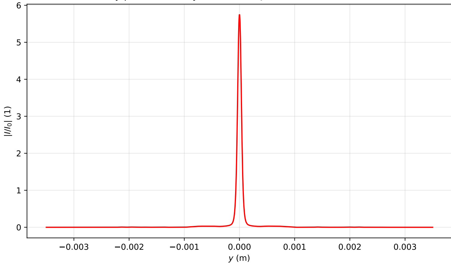
Intensity profile I(x = 0, y, z = 2.149)/I_0 , P_{in}=16.5P_{cr} , artificial time
