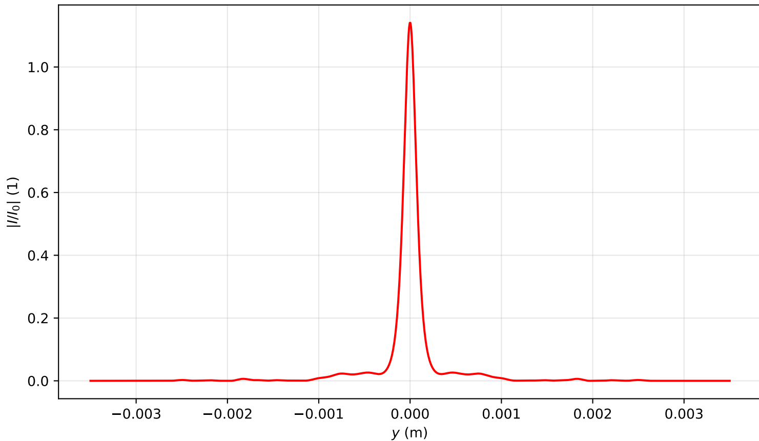
Intensity profile I(x=0, y, z=2.388)/I_0 , P_{in}=16.5P_{cr} , artificial time
