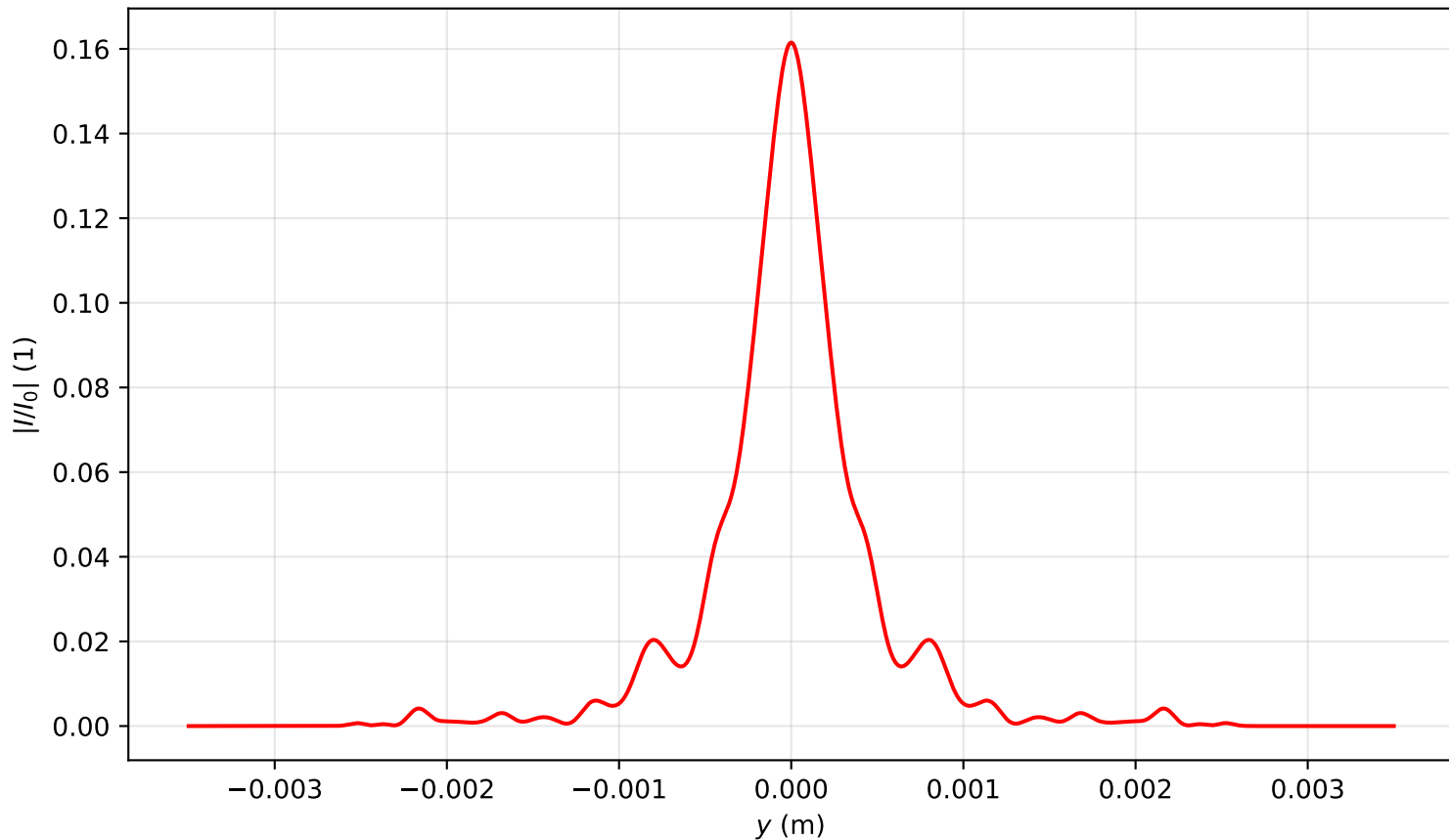
Intensity profile I(x=0, y, z=2.627)/I_0 , P_{in}=16.5P_{cr} , artificial time
