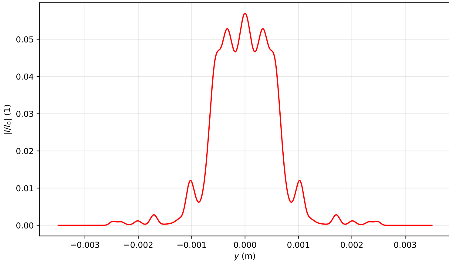
Intensity profile I(x=0, y, z=2.866)/I_0 , P_{in}=16.5P_{cr} , artificial time
