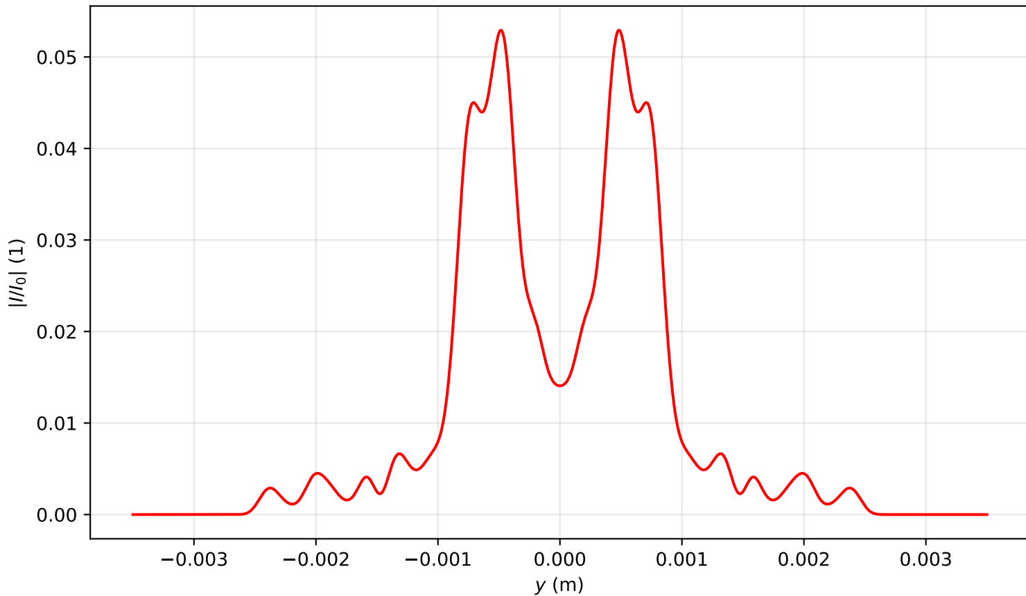
Intensity profile I(x=0, y, z=3.105)/I_0 , P_{in}=16.5P_{cr} , artificial time
