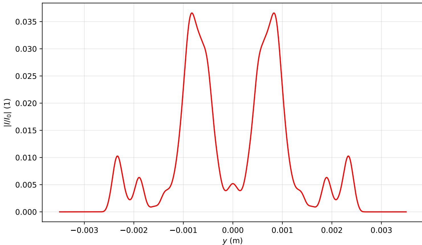
Intensity profile I(x=0, y, z=3.582)/I_0 , P_{in}=16.5P_{cr} , artificial time
