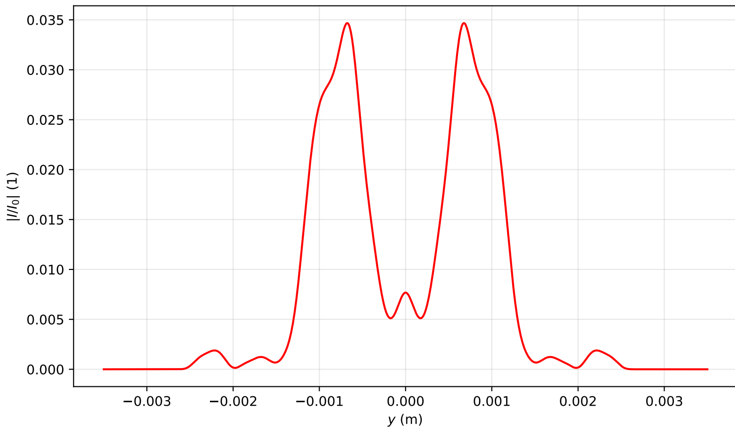
Intensity profile I(x=0, y, z=3.821)/I_0 , P_{in}=16.5P_{cr} , artificial time
