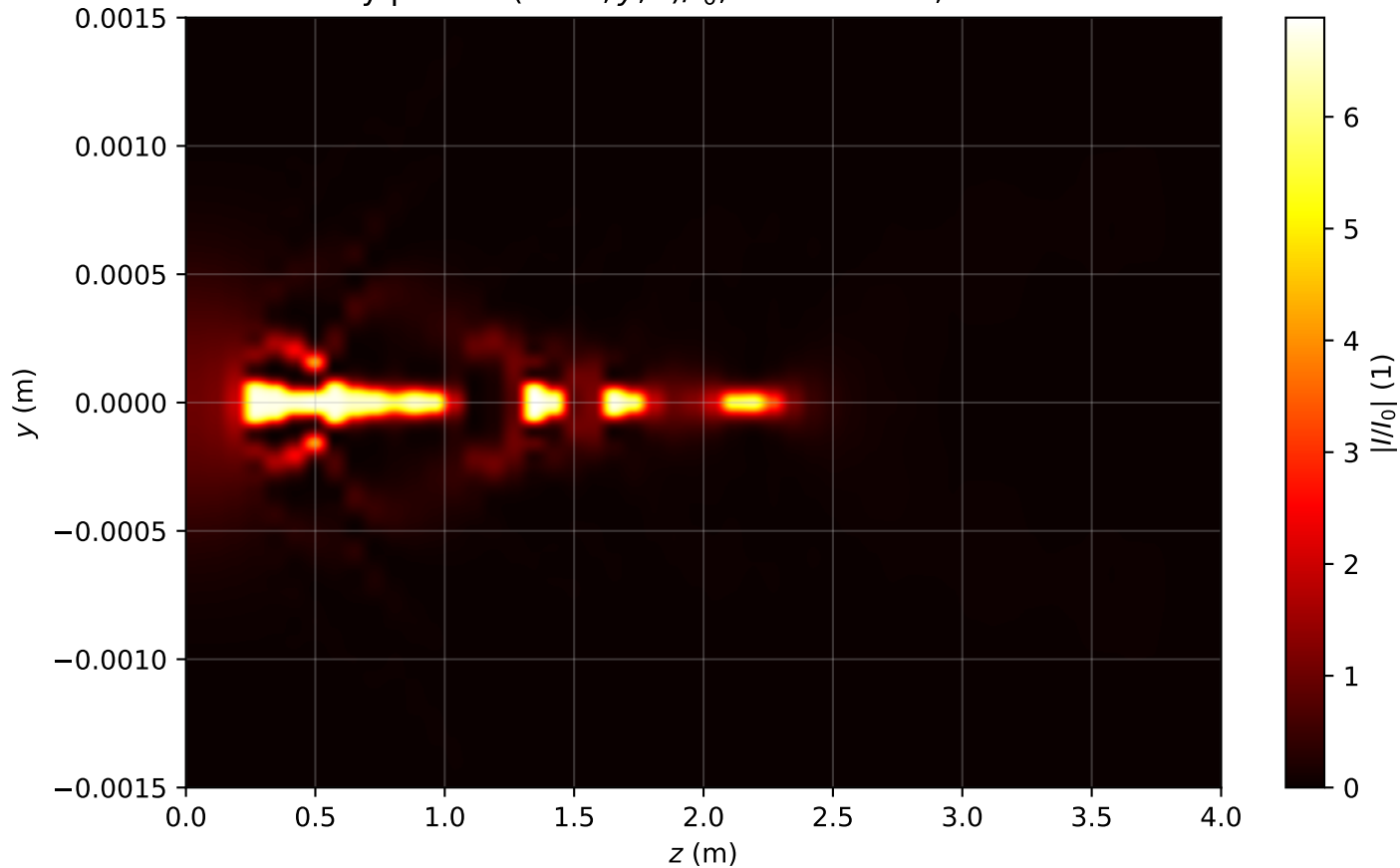
Intensity profile I(x=0, y, z)/I_0 , P_{in}=16.5P_{cr} , artificial time
