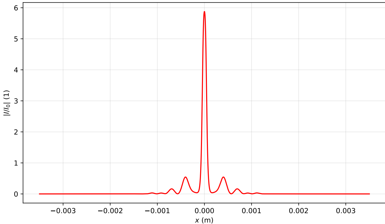
Intensity profile I(x, y = 0, z = 0.716)/I_0 , P_{in}=18.0P_{cr} , artificial time
