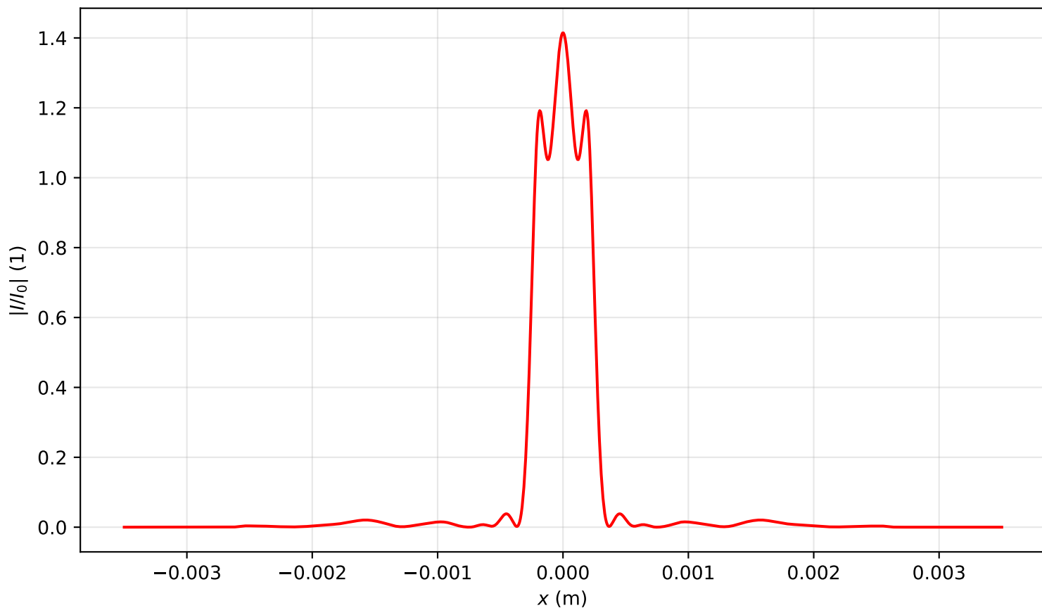
Intensity profile I(x, y = 0, z = 1.194)/I_0 , P_{in}=18.0P_{cr} , artificial time
