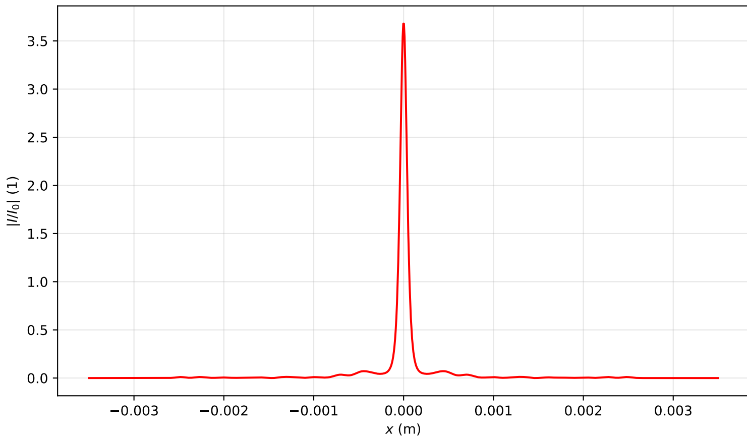
Intensity profile I(x, y = 0, z = 1.672)/I_0 , P_{in}=18.0P_{cr} , artificial time
