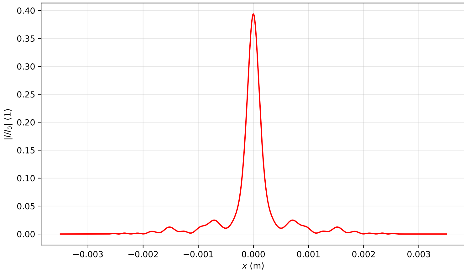
Intensity profile I(x, y = 0, z = 2.388)/I_0 , P_{in}=18.0\text{Pcr} , artificial time
