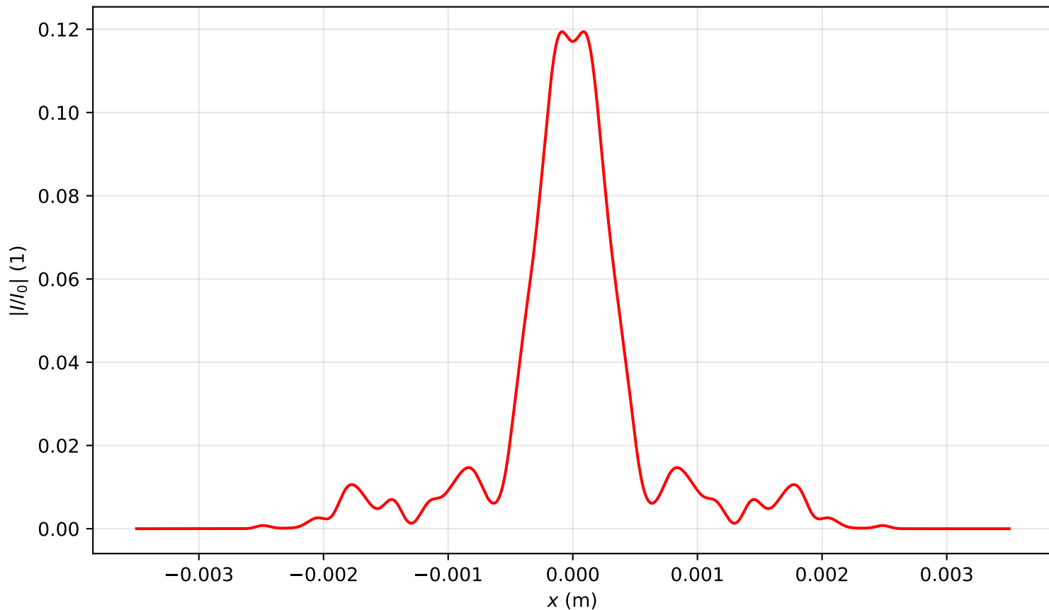
Intensity profile I(x, y = 0, z = 2.627)/I_0 , P_{in}=18.0\text{Pcr} , artificial time
