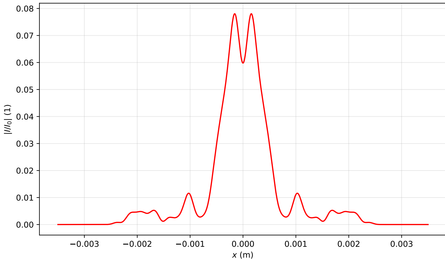
Intensity profile I(x, y = 0, z = 2.866)/I_0 , P_{in}=18.0P_{cr} , artificial time
