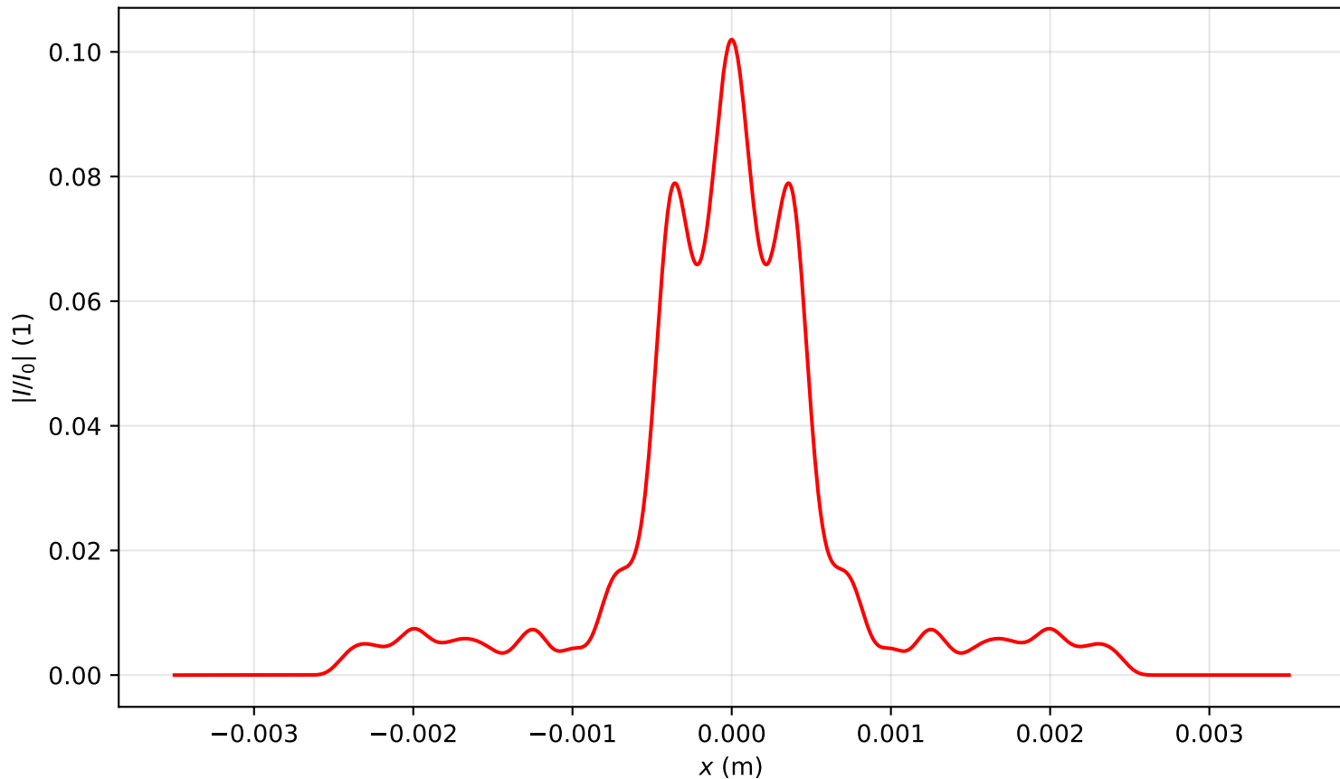
Intensity profile I(x, y = 0, z = 3.105)/I_0 , P_{in}=18.0\text{Pcr} , artificial time
