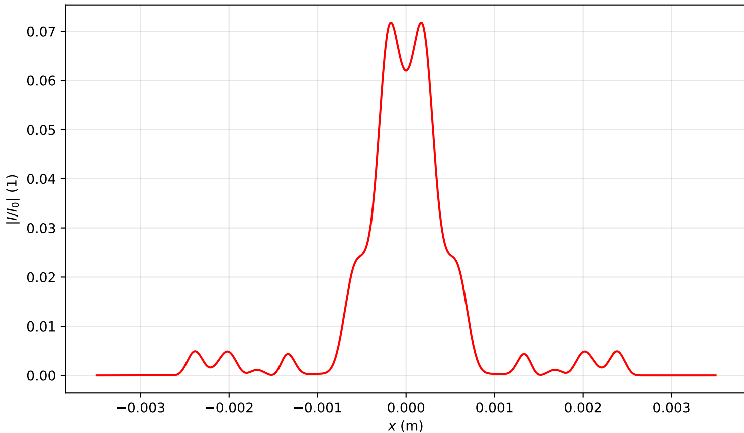
Intensity profile I(x, y = 0, z = 3.344)/I_0 , P_{in}=18.0\text{Pcr} , artificial time
