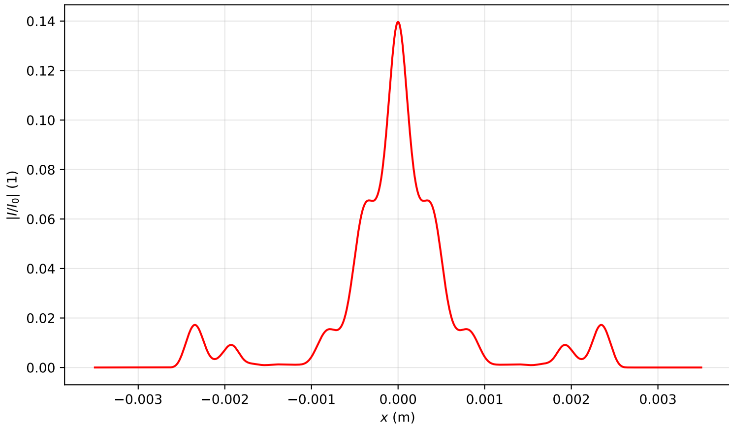
Intensity profile I(x, y = 0, z = 3.582)/I_0 , P_{in}=18.0\text{Pcr} , artificial time
