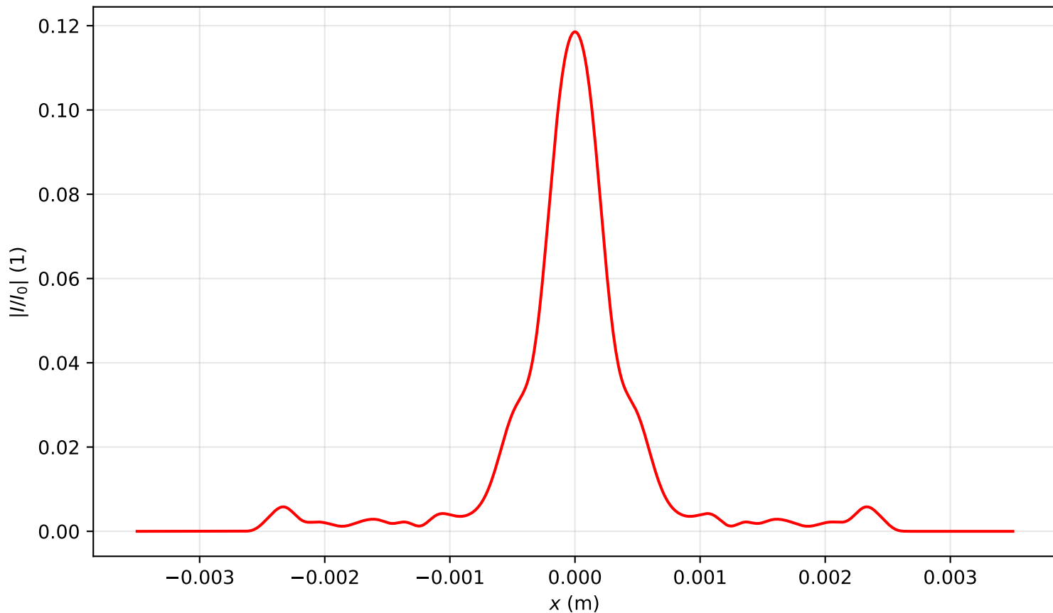
Intensity profile I(x, y = 0, z = 3.821)/I_0 , P_{in}=18.0\text{Pcr} , artificial time
