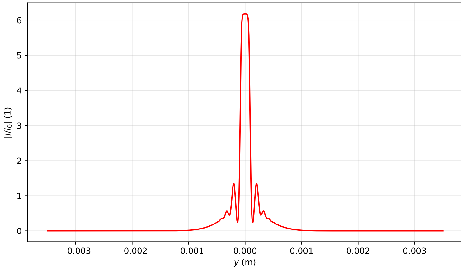
Intensity profile I(x = 0, y, z = 0.239)/I_0 , P_{in}=18.0P_{cr} , artificial time
