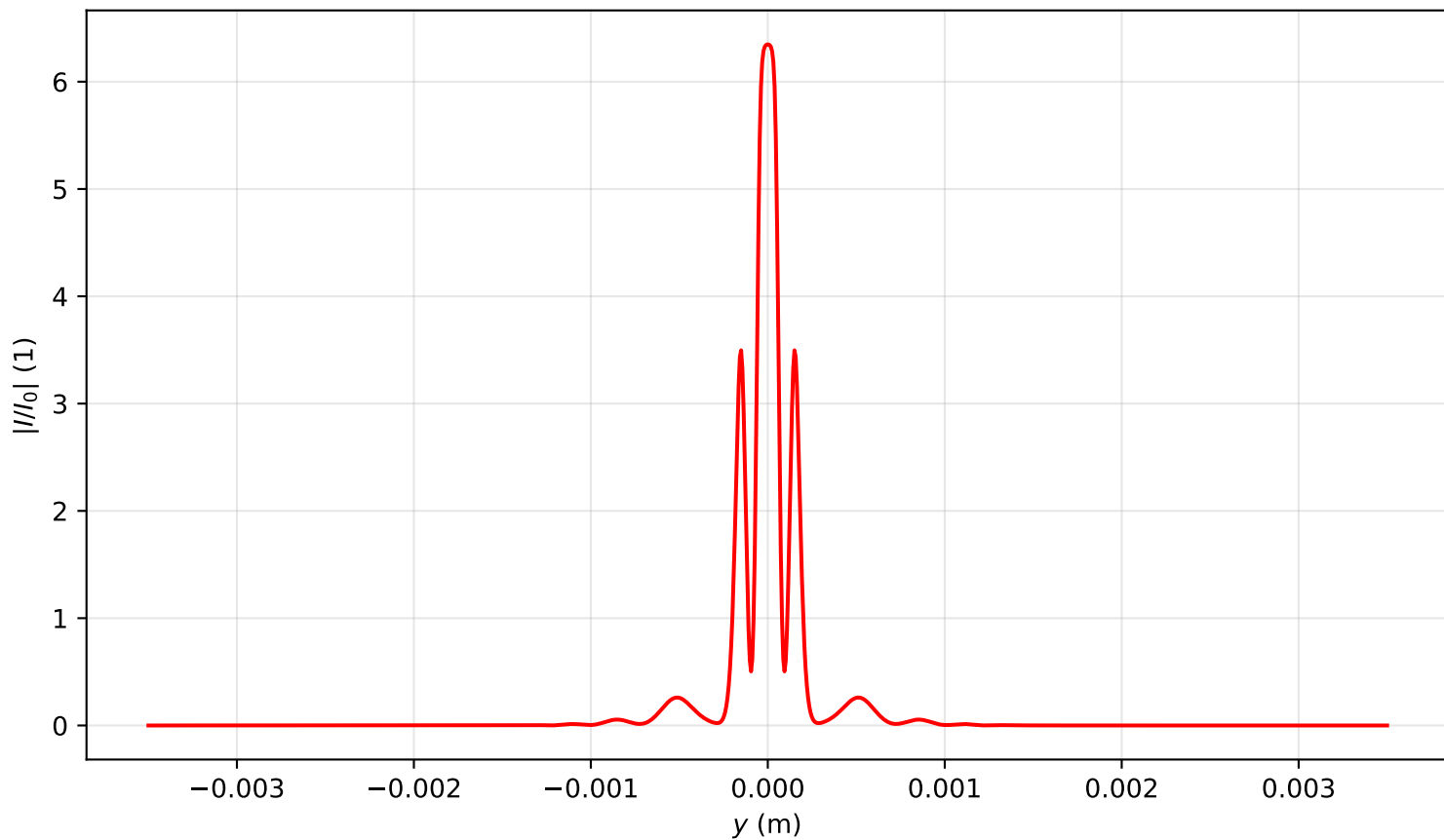
Intensity profile I(x=0, y, z=0.478)/I_0 , P_{in}=18.0P_{cr} , artificial time
