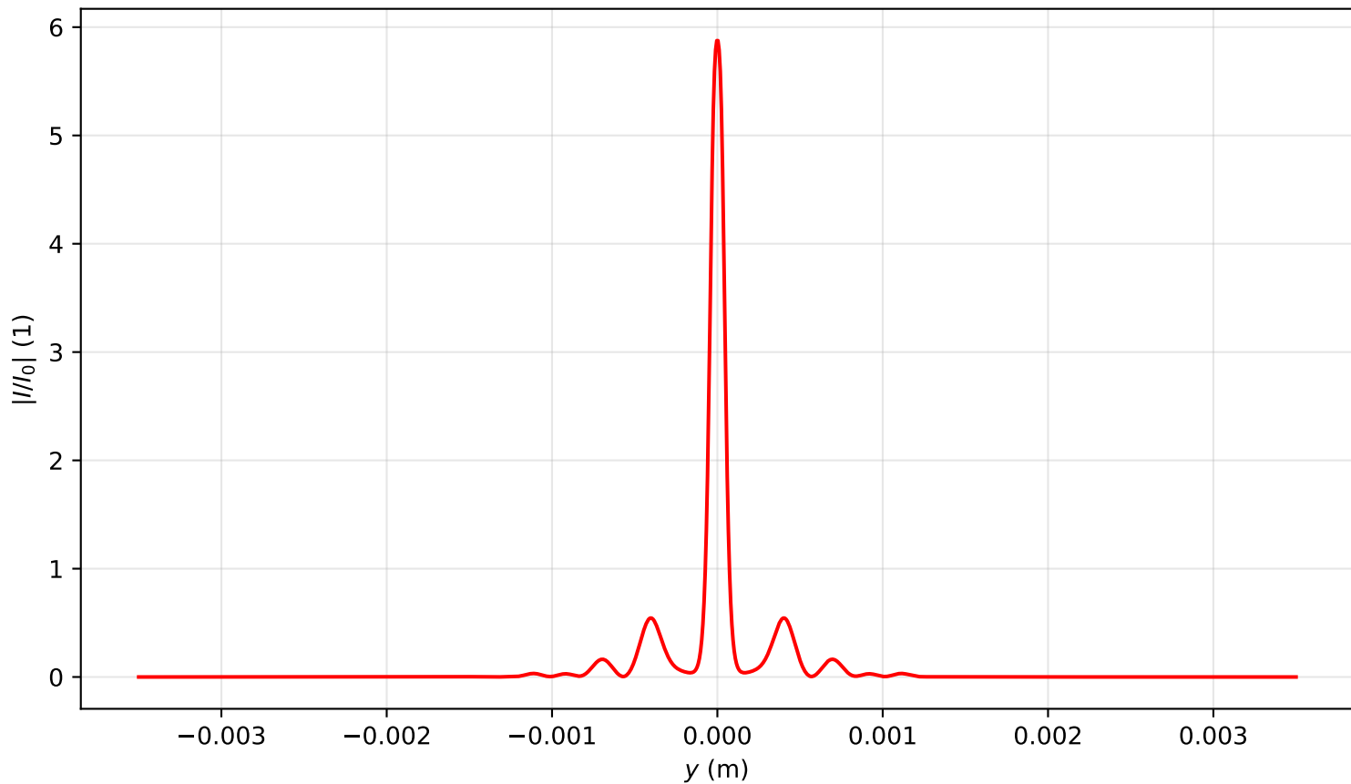
Intensity profile I(x = 0, y, z = 0.716)/I_0 , P_{in}=18.0\text{Pcr} , artificial time
