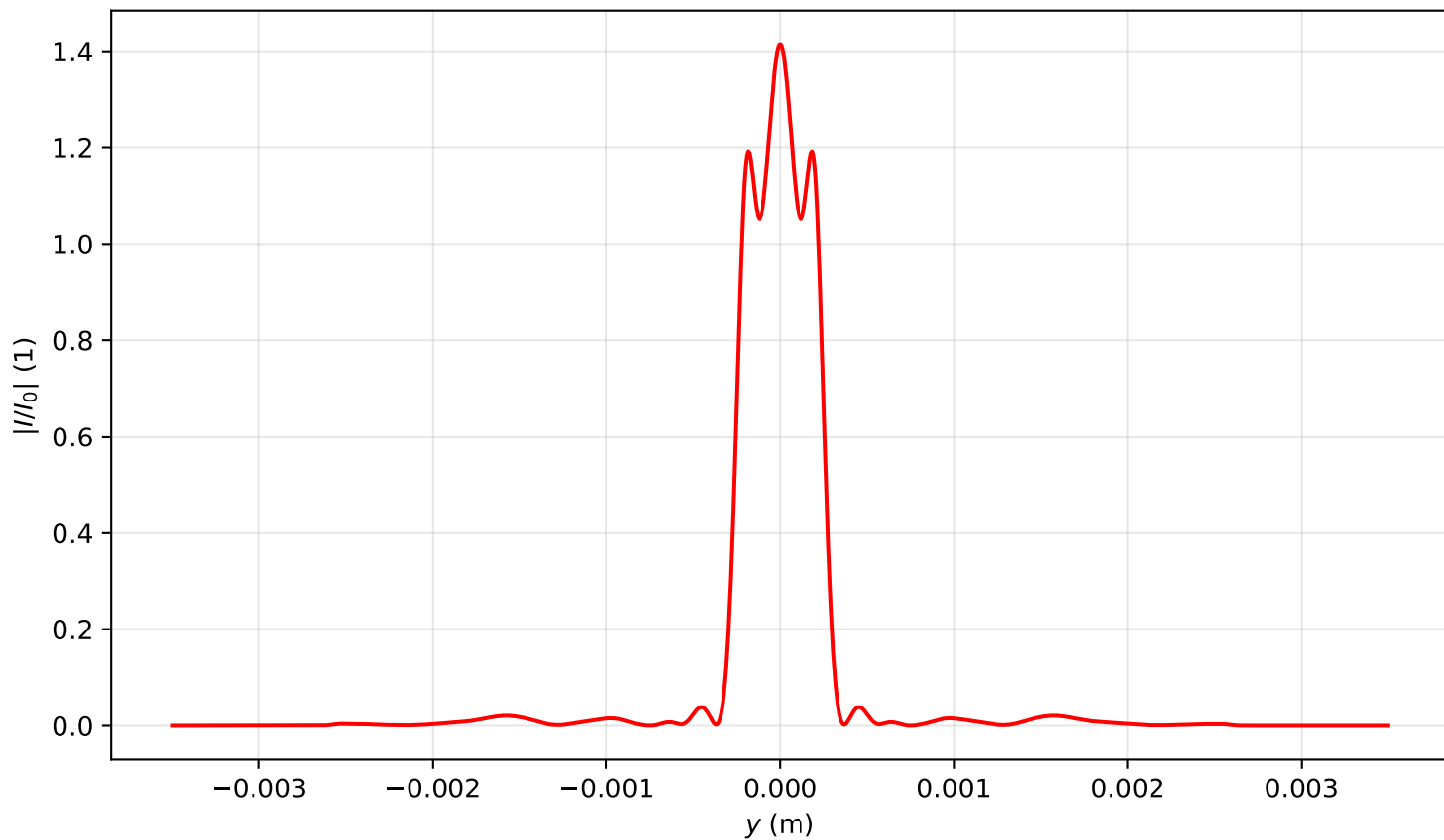
Intensity profile I(x=0, y, z=1.194)/I_0 , P_{in}=18.0P_{cr} , artificial time
