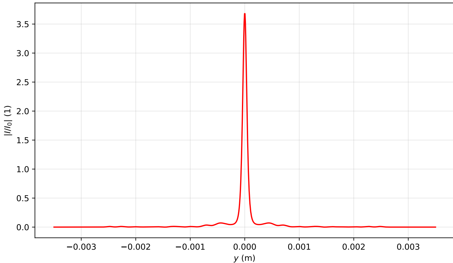
Intensity profile I(x=0, y, z=1.672)/I_0 , P_{in}=18.0P_{cr} , artificial time
